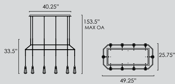
SM23787 • Linear Chandelier
