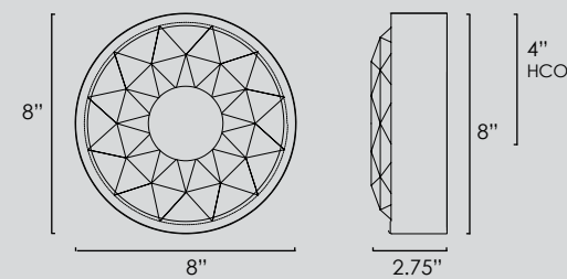
SM24851 • Round Sconce
