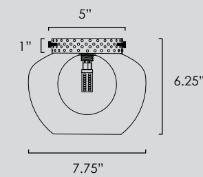
SM31080 • Flush Mount
