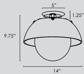
SM31009 • Flush Mount
