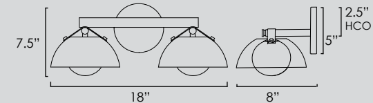
SM31002 • Bath Vanity
