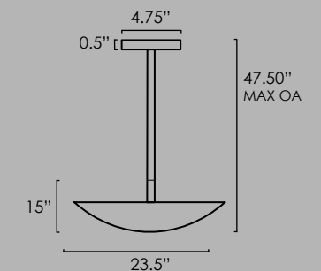
SM81854 • 24" LED Pendant/Semi-Flush
