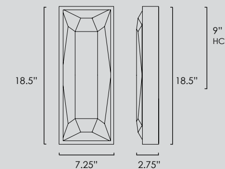
SM24853 • Wall Sconce
