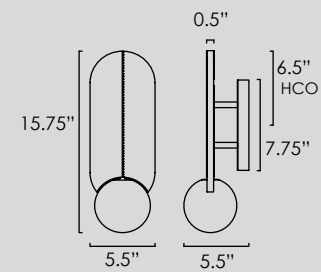
SM24601 • Down-Light Wall Sconce
