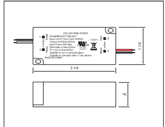
LED DRIVER DIAGRAM
